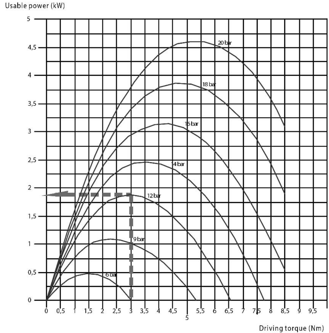
Graph nb 2 : Usable power depending on driving torque.
