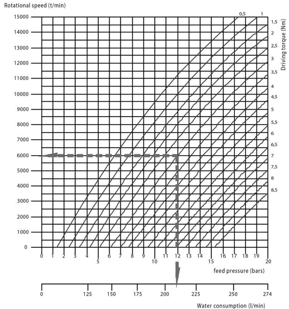
Graph nb 1 : Rotational speed and water consumption depending on feed pressure.
